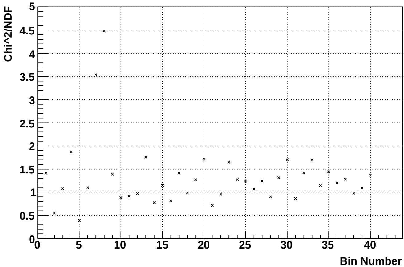
Chi Squared vs. Bin Number, Before Gap
