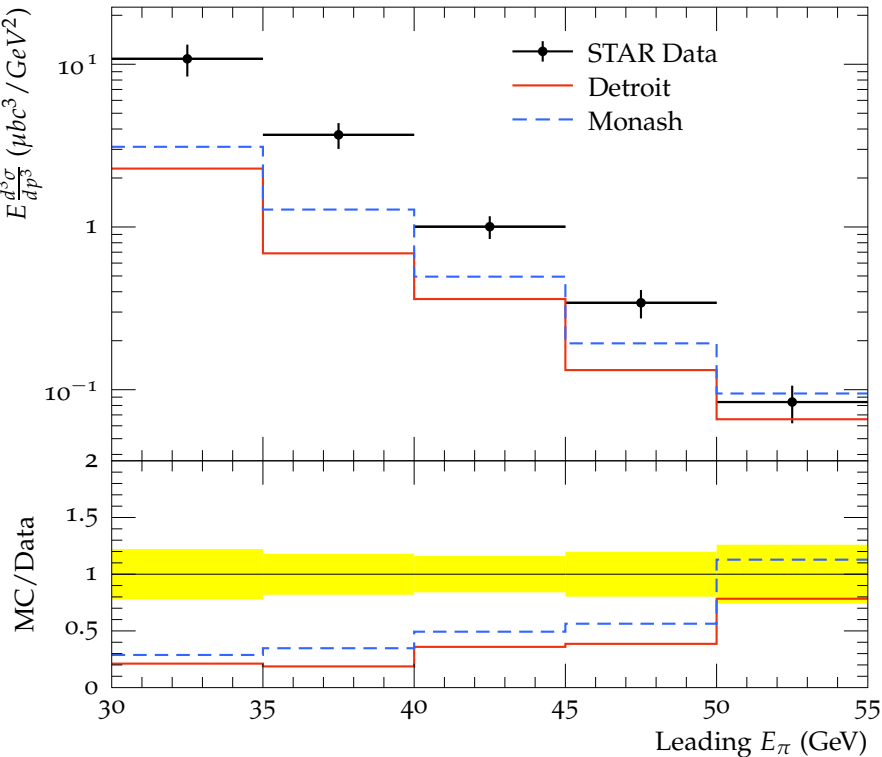
Inclusive \pi^0 Cross Section vs Leading E_\pi in 3.4 < \eta < 4
